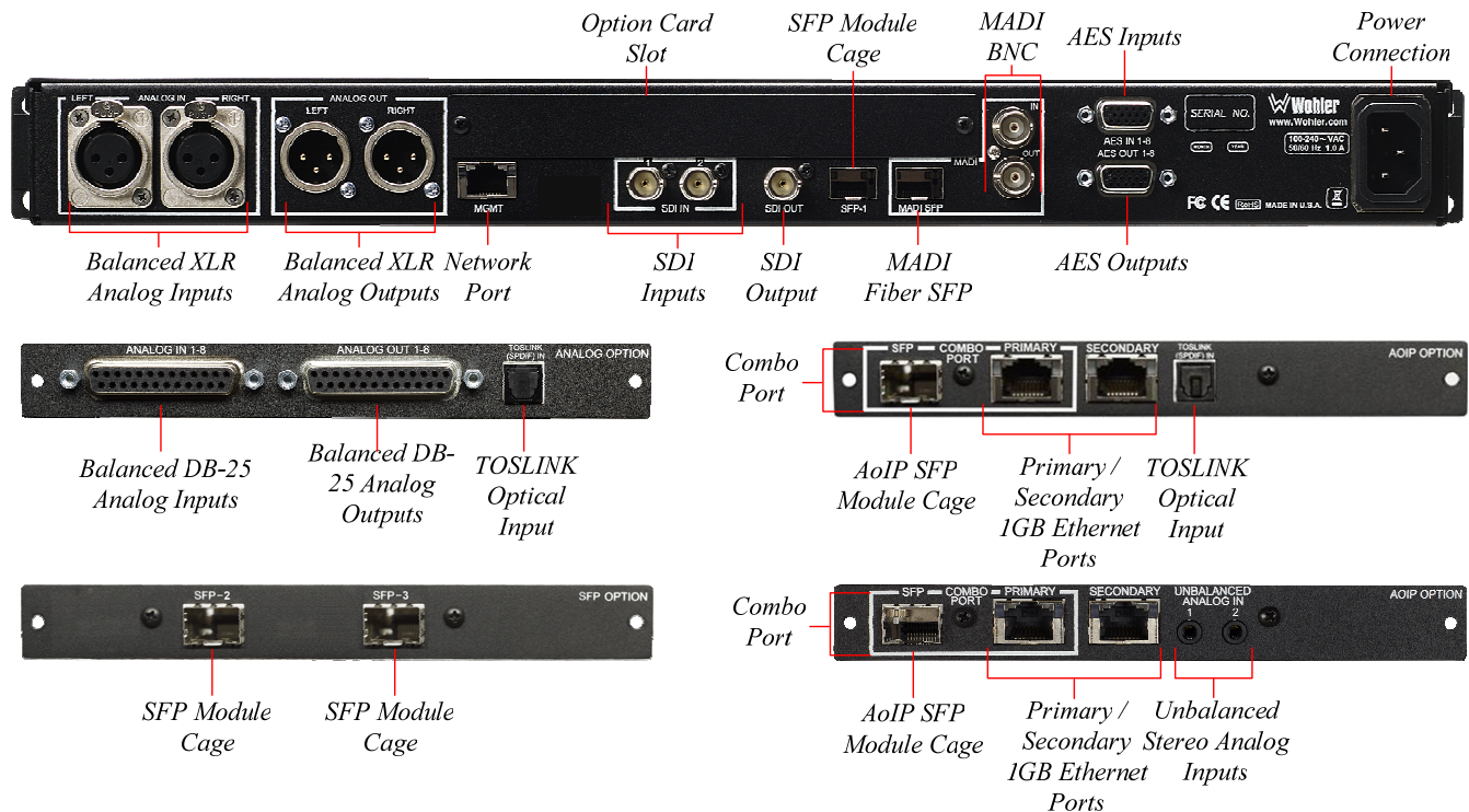
Figure 2-2: iAM1-12G Rear Panel & Option Cards
