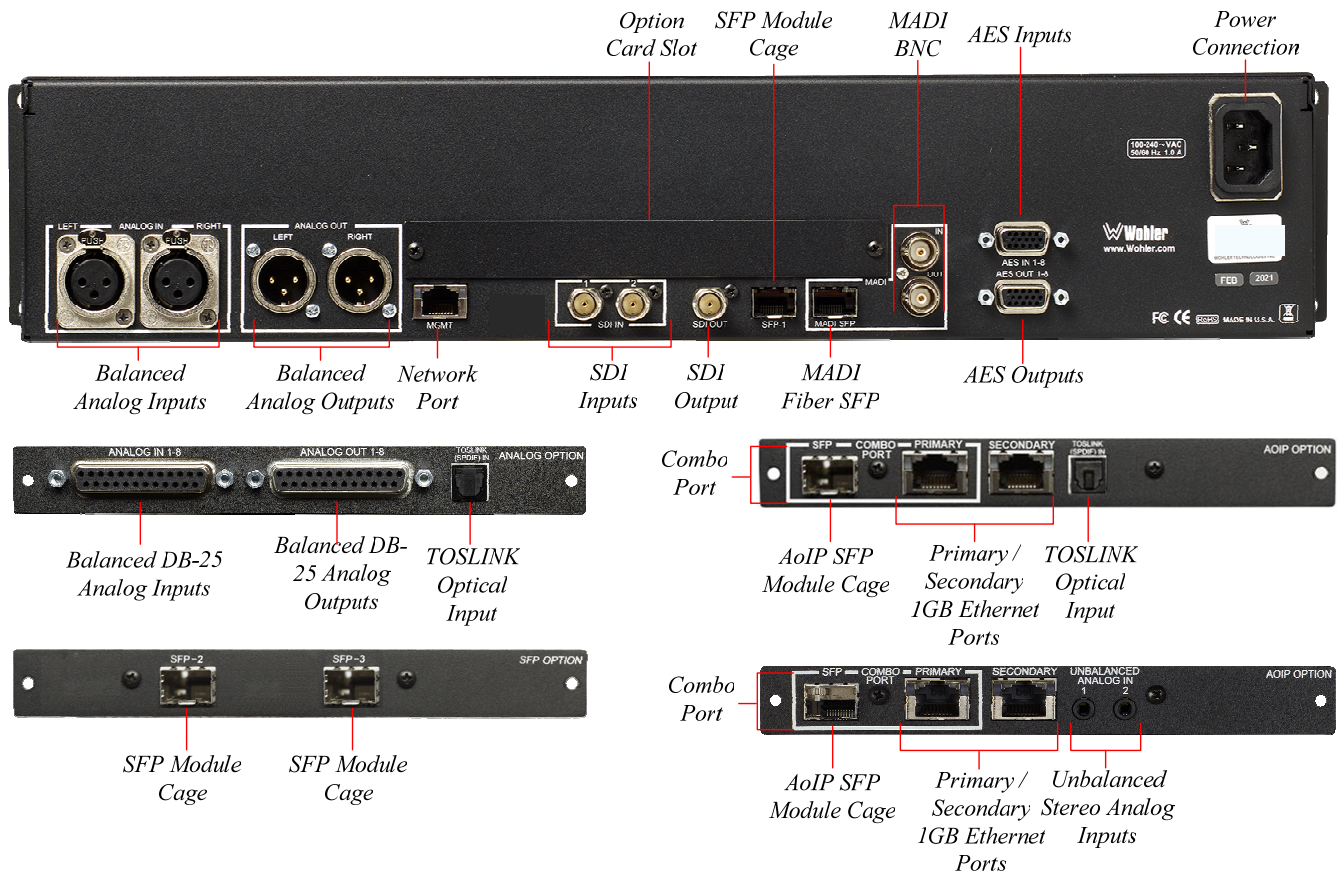
Figure 2-2: iVAM2-2 Rear Panel & Option Cards
