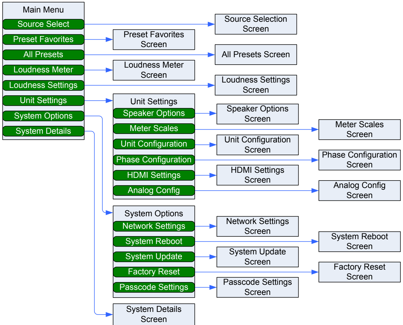
Figure 2-11: Menu Tree
