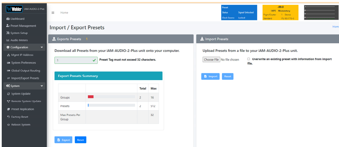
Figure 4-24: Database Export
