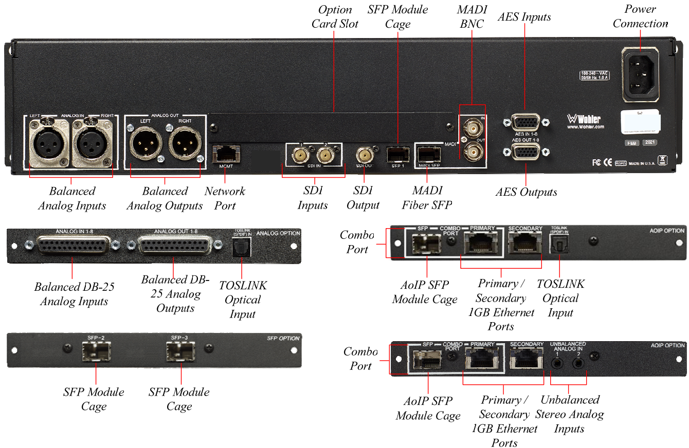
Figure 2-2: iAM-AUDIO-2 PLUS Rear Panel & Option Cards
