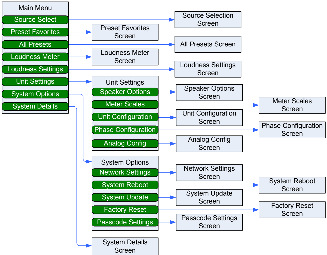
Figure 2-10: Menu Tree
