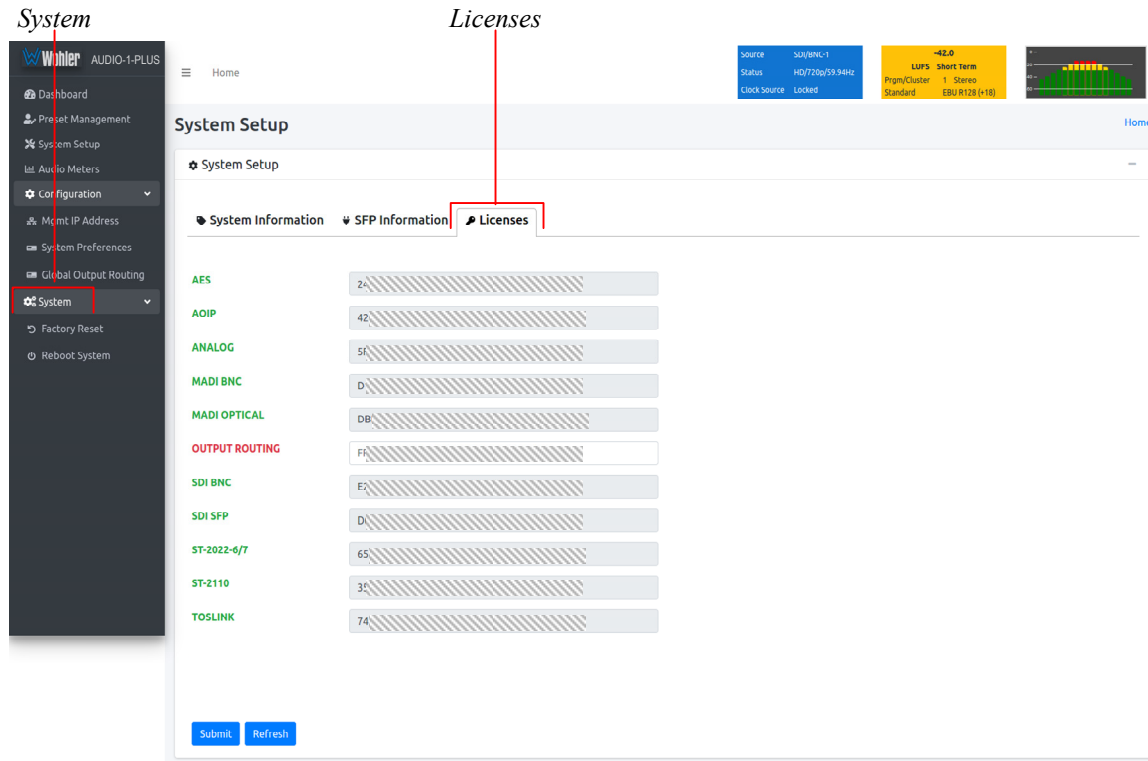
Figure 4-24: Licenses Tab
