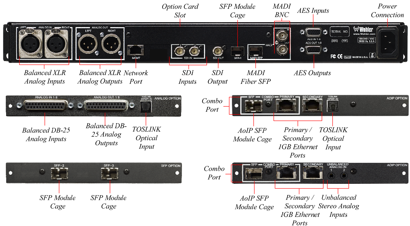
Figure 2-2: iAM-AUDIO-1 PLUS Rear Panel & Option Cards
