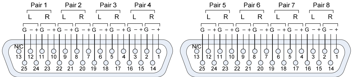
Figure 1-4: Balanced Analog Input XLR-F Pin Out
