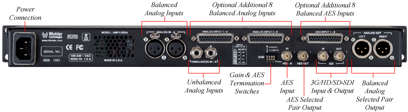
Figure 1-2: Rear Panel Layout
