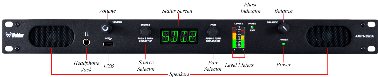
Figure 1-1: Front Panel Layout
