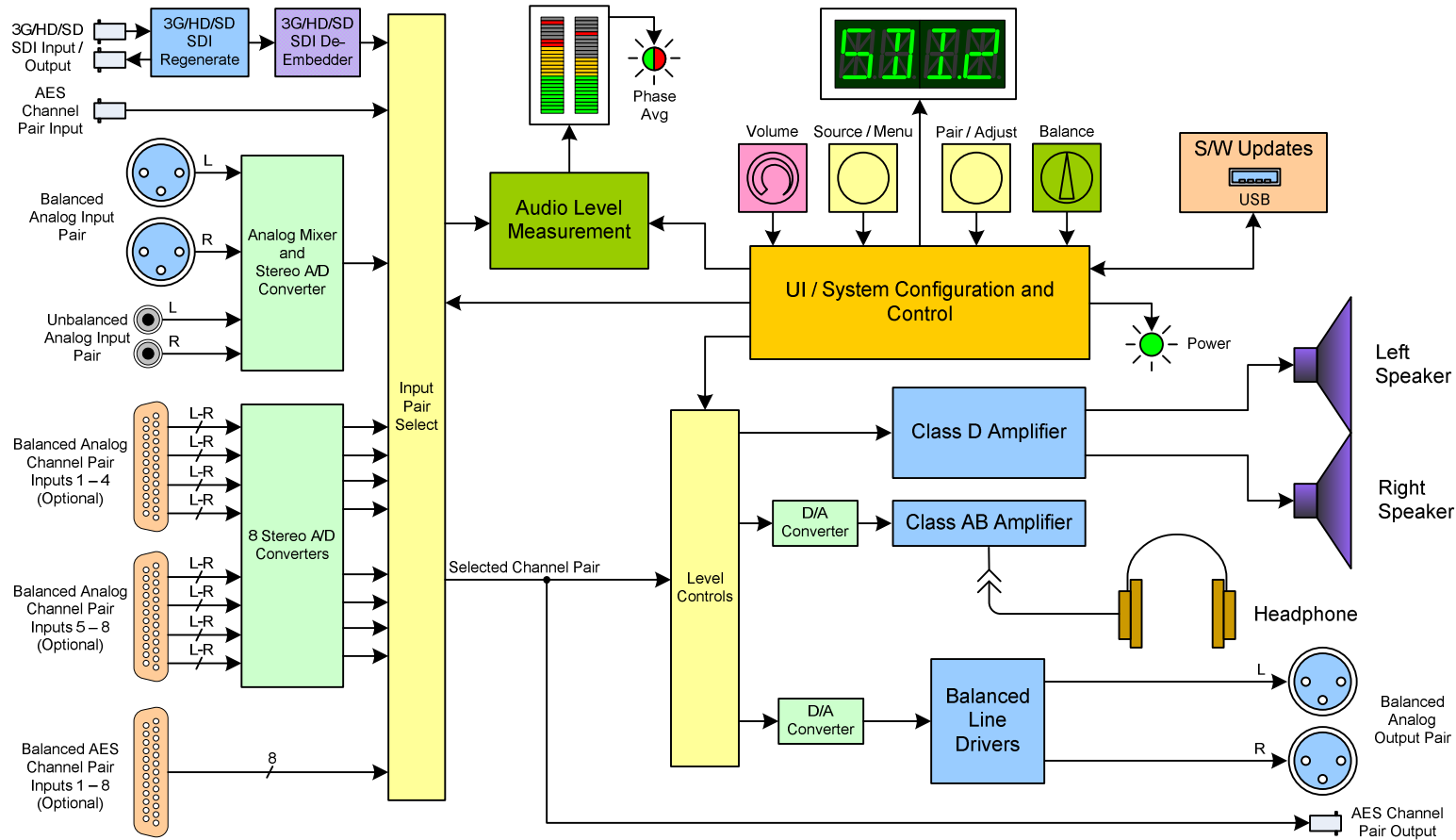
Figure 4-1: AMP1-2SDA Block Diagram
