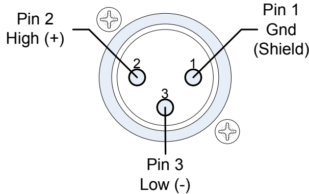
Figure 1-3: Balanced Analog Input XLR-F Pin Out
