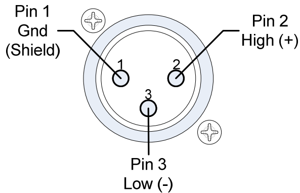
Figure 1-6: Balanced Analog Output XLR-M Pin Out
